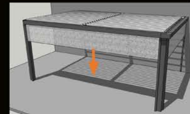
Surface-mounted Zip blind (box fixed against the crossbars on the outside)
